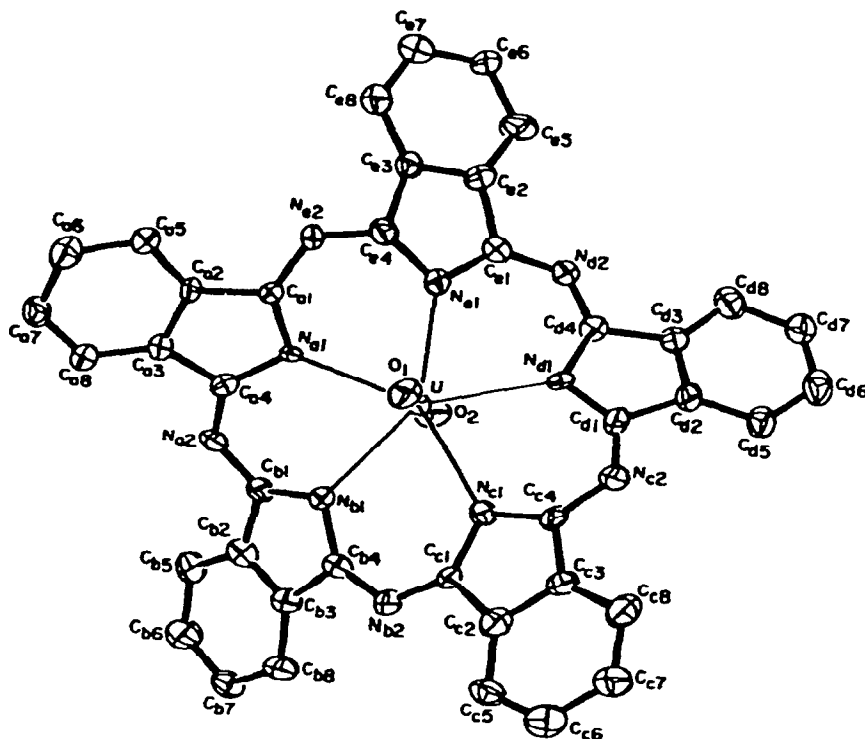
Fig. 6. Structure of uranilsuperphthalocyanine [30].
