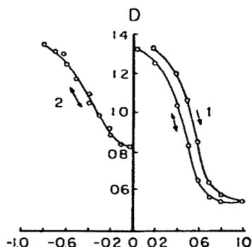
Fig. 10. Variation of the steady-state optical density of the lutetium-diphthalocyanine film with electrode potential: (1) at 673 nm; (2) at 640 nm. The arrows against the curves indicate the direction of measurements on the potential scale [77].
