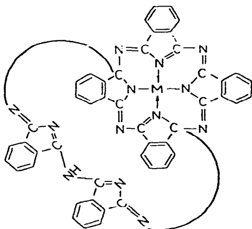
Fig. 5. Proposed metallophthalocyanine precursors. M = \text{Ni(II)} or \text{Cu(II)} .
