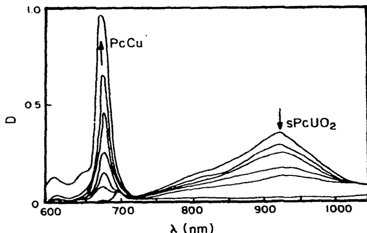
Fig. 7. The reaction of uranylsuperphthalocyanine with \text{CuCl}_2 in 300/1 = 1-chloronaphthalene/DMF at 75^\circ\text{C} [31].
